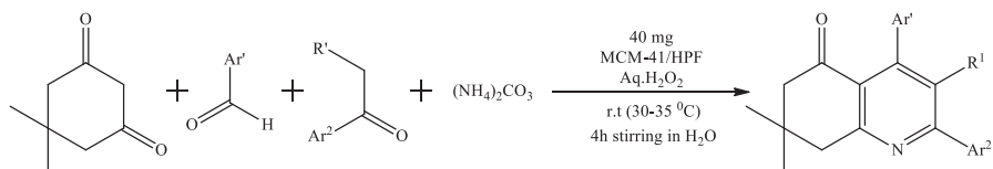
Scheme 2.1.2.2.4
