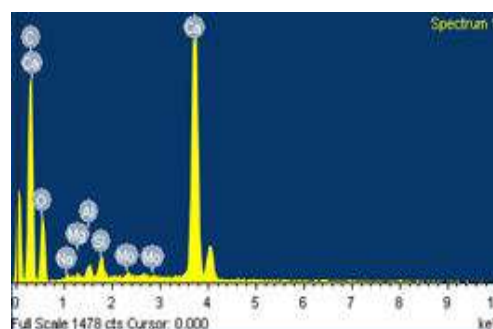
Fig. 7 Elemental Spectrum
