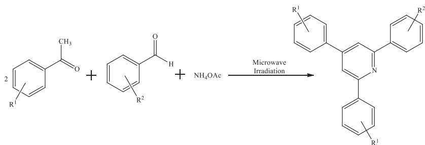
Scheme 2.1.2.2
