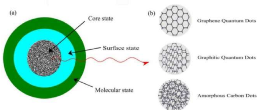
Figure 2: (a) Carbon dot structure and (b) carbon dot structural core analysis.
