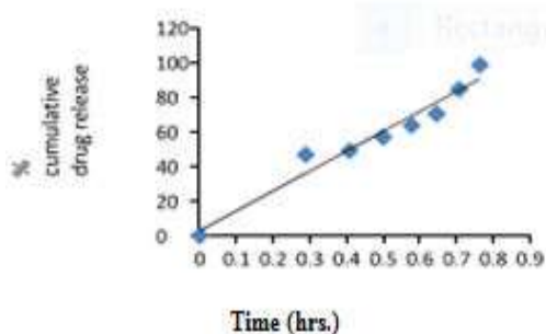
Figure 8: Higuchi Curve
