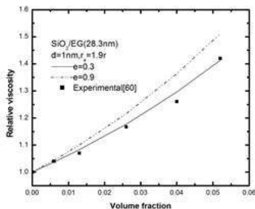
Figure 3(b): The variation of relative viscosity with volume fraction for SiO 2 /EG nanofluid for d p =28.3nm for different eccentricity
