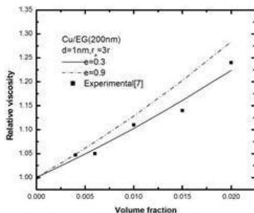
Figure 5(b): The variation of relative viscosity with volume fraction for Cu/EG for d_p=200\text{nm} for different eccentricity
