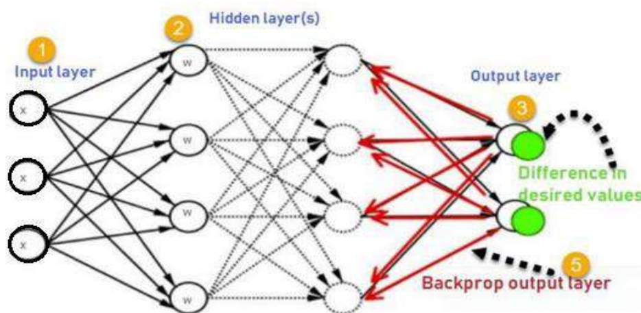
Figure-3 Optimized FFBPNN
