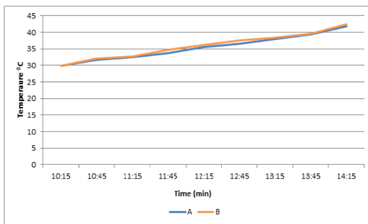
Fig. 2.18 Temperature Variations for High Flowing Rates
