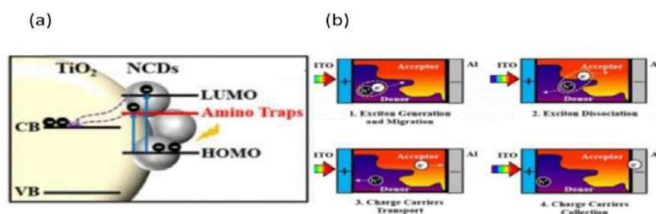
Figure 19: (a) A proposed framework for photo-induced electron transfer between NCDs and TiO 2 [216,217] and (b) the energy generating steps in a BHJ-OSC cell.
