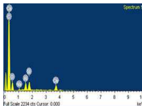
Fig. 5 Elemental Spectrum
