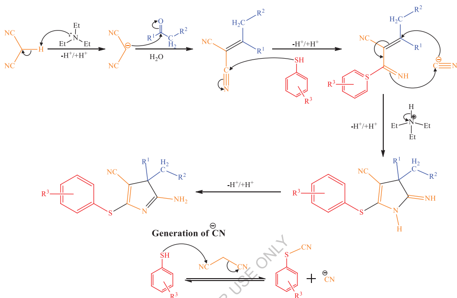
Scheme 2.2.3 Probable mechanism of 3 H -pyrrole formation
