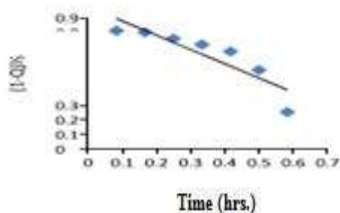
Figure 9: Hixon Crowell Plot
