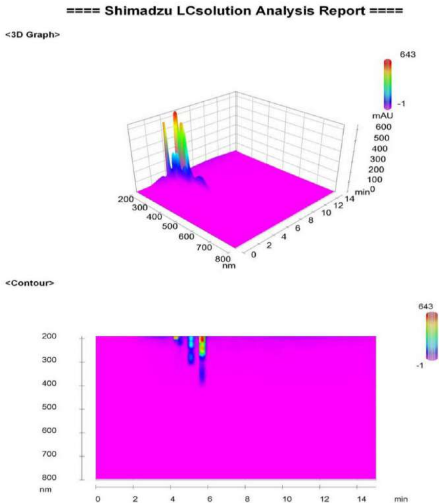
Figure 5: 3D graph and counter graph of cilnidipine analysis
