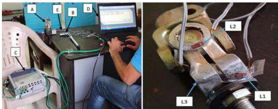
a) Experimental setup b) Strain gauges locating positions
