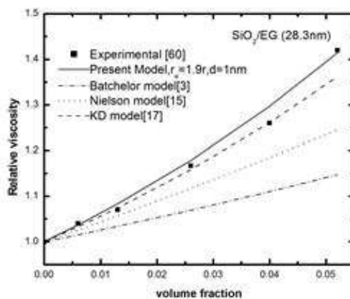
Figure 3(a): The variation of relative viscosity with volume fraction for SiO 2 /EG nanofluid for d p =28.3nm
