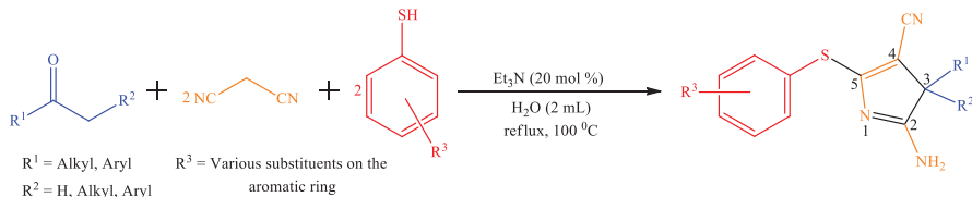
Scheme 2.2.1
