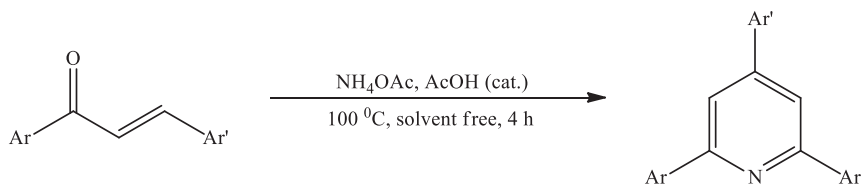
Scheme 2.1.2.2.1
