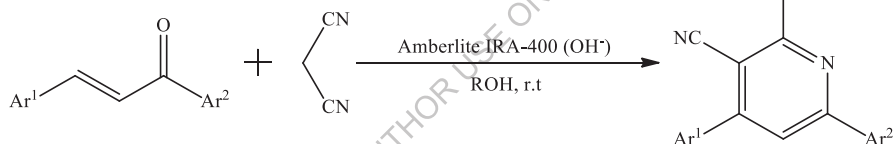
Scheme 2.1.2.2.5
